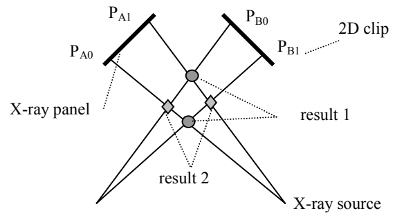
Figure 4. Back-projection with two possible results
