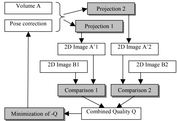
Figure 6. Algorithm for grey value based six degrees of freedom registration
